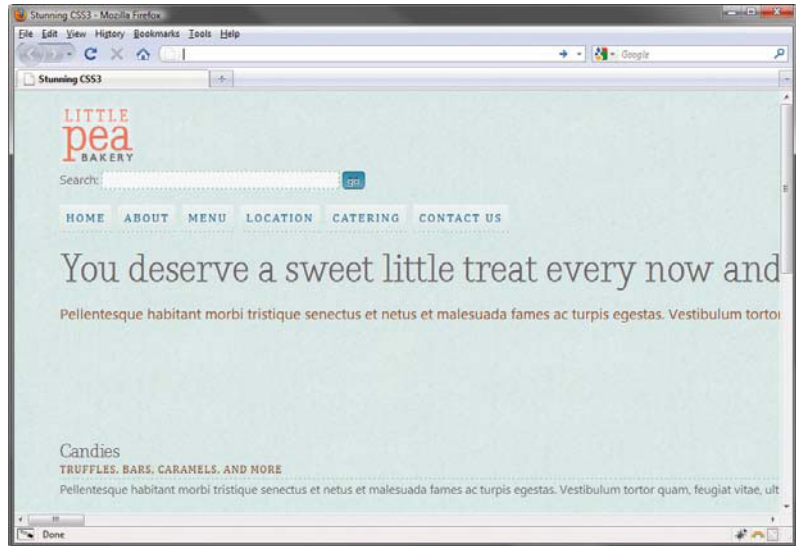
FIGURE 7.2 The two content divs are now placed side by side, but overflow tremendously off the right side of the viewport.
