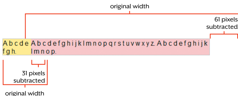
FIGURE 7.7 The pink div has 61 pixels subtracted from it, while the yellow one has only 31 pixels subtracted, since their box-flex values are in a two-to-one ratio.
