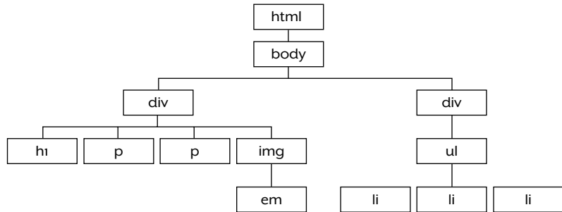
FIGURE 5.1 A sample document tree, showing ancestor, descendant, parent, child, and sibling elements
